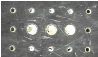
Figure 6: Unfilled vias
